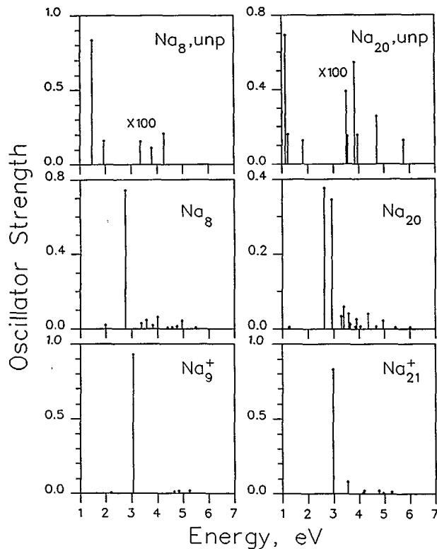
FIG. 2. Oscillator strength function for the photoabsorption of \text{Na}_8 , \text{Na}_{20} , \text{Na}_9^+ , and \text{Na}_{21}^+ clusters. In the upper figures, the unperturbed oscillator strengths for the neutral clusters is displayed. Also, in the upper figures, the strength values above 3 eV have been multiplied by 100.
