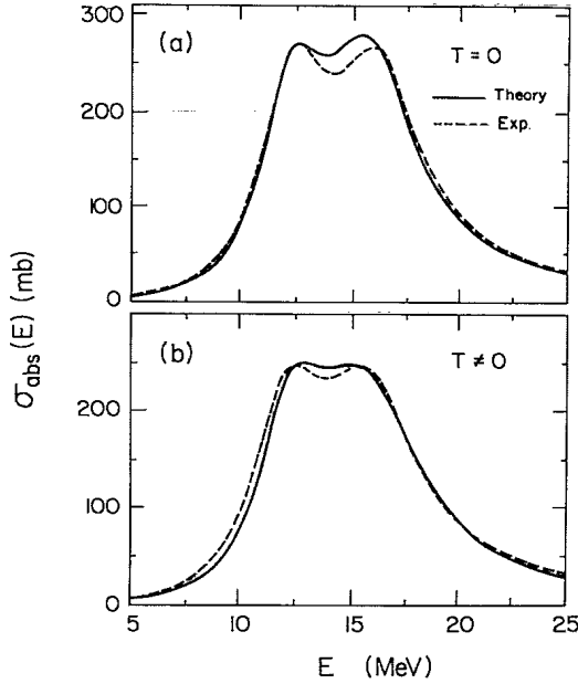
FIG. 3. The experimental results at (a) T=0 and (b) T \neq 0 were taken from Refs. 14 and 19, and are displayed as a dashed curve. The full line in (a) gives the results of the present calculation for the ground state of ^{166}\text{Er} . The full line in (b) gives the results of the present calculation for the same nucleus and for T \neq 0 (cf. Ref. 20) and \omega=0.2 MeV, which corresponds to an angular momentum I=15\hbar . The rotational frequency \omega and angular momentum I are related according to Ref. 1.
