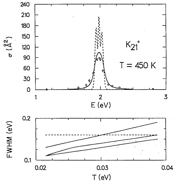
FIG. 2. Quantal size effects for K_{21}^+ : Lower part: Results for the FWHM obtained using Eqs. (1)–(4), and taking for \Gamma in Eq. (1) the parametrization of Eq. (5) with \gamma=1 (lower curve), \gamma=2 (middle curve), and \gamma=3 (upper curve). The horizontal dashed line corresponds to the experimentally determined FWHM for the range of possible temperatures of the cluster (Ref. 22). Upper part: Photoabsorption cross section. The experimental data (Ref. 6) are plotted with open circles; the dashed line displays the resulting broadening due solely to thermal fluctuations (zero intrinsic width). The full drawn curve includes the relaxation process (i) (cf. text), using the parametrization in Eq. (5) with \gamma=2 . The temperature selected corresponds to the crossing point between the middle solid and the horizontal dashed curves in the lower part of this figure.
