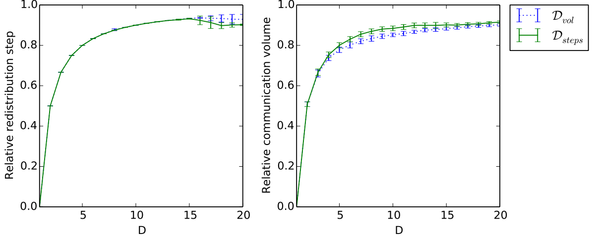
Figure 2: Performance of \mathcal{D}_{vol} (computed by Algorithm ??) and \mathcal{D}_{steps} (computed by Algorithm ??) relatively to the canonical distribution, for a random initial distribution and for both metrics.
